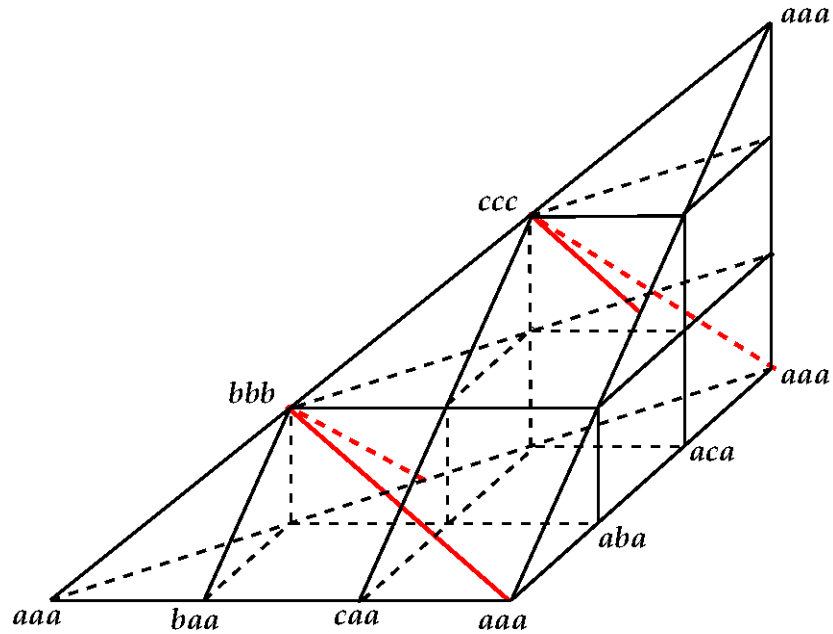
Figure 8: A 3-fold symmetric product of the triangle curve with the image of the curve in marked.
