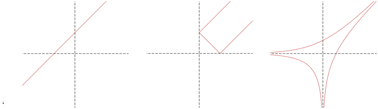
Figure 1: The image of the line under (x, y) \mapsto (|x|, |y|) \mapsto (\log_t |x|, \log_t |y|) .
